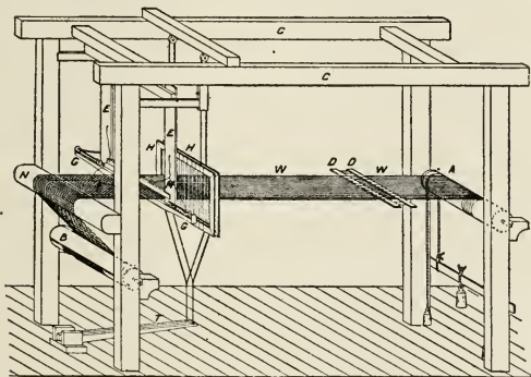
DIAGRAM OF A HAND LOOM
